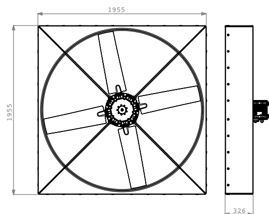
WA1800
